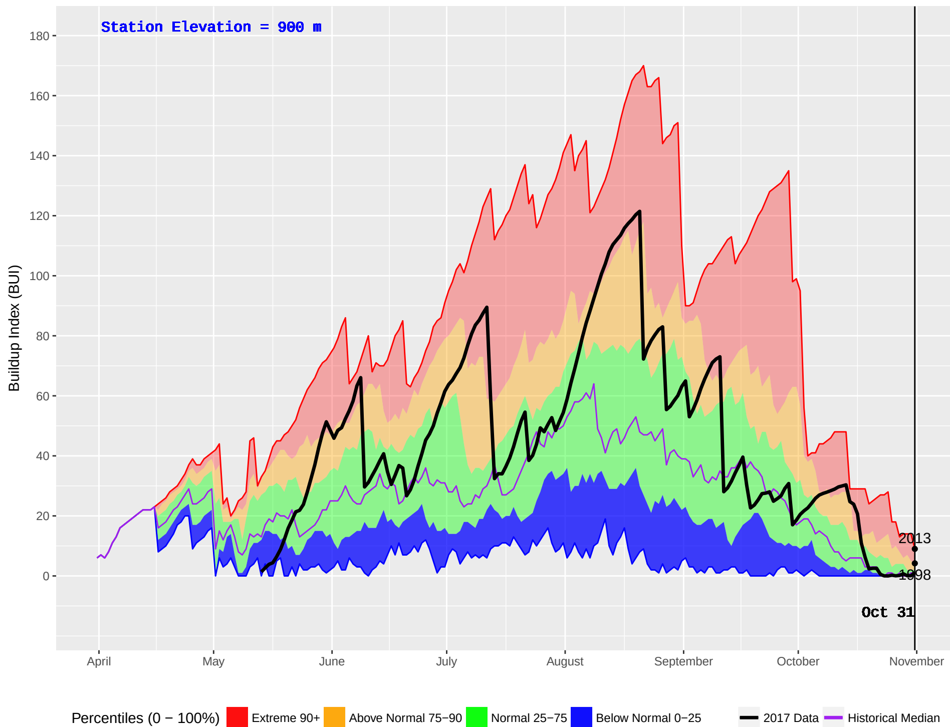
UPPER FULTON (169) : Historical (1986–2016) and Current (2017) Noon Buildup Index (BUI)
