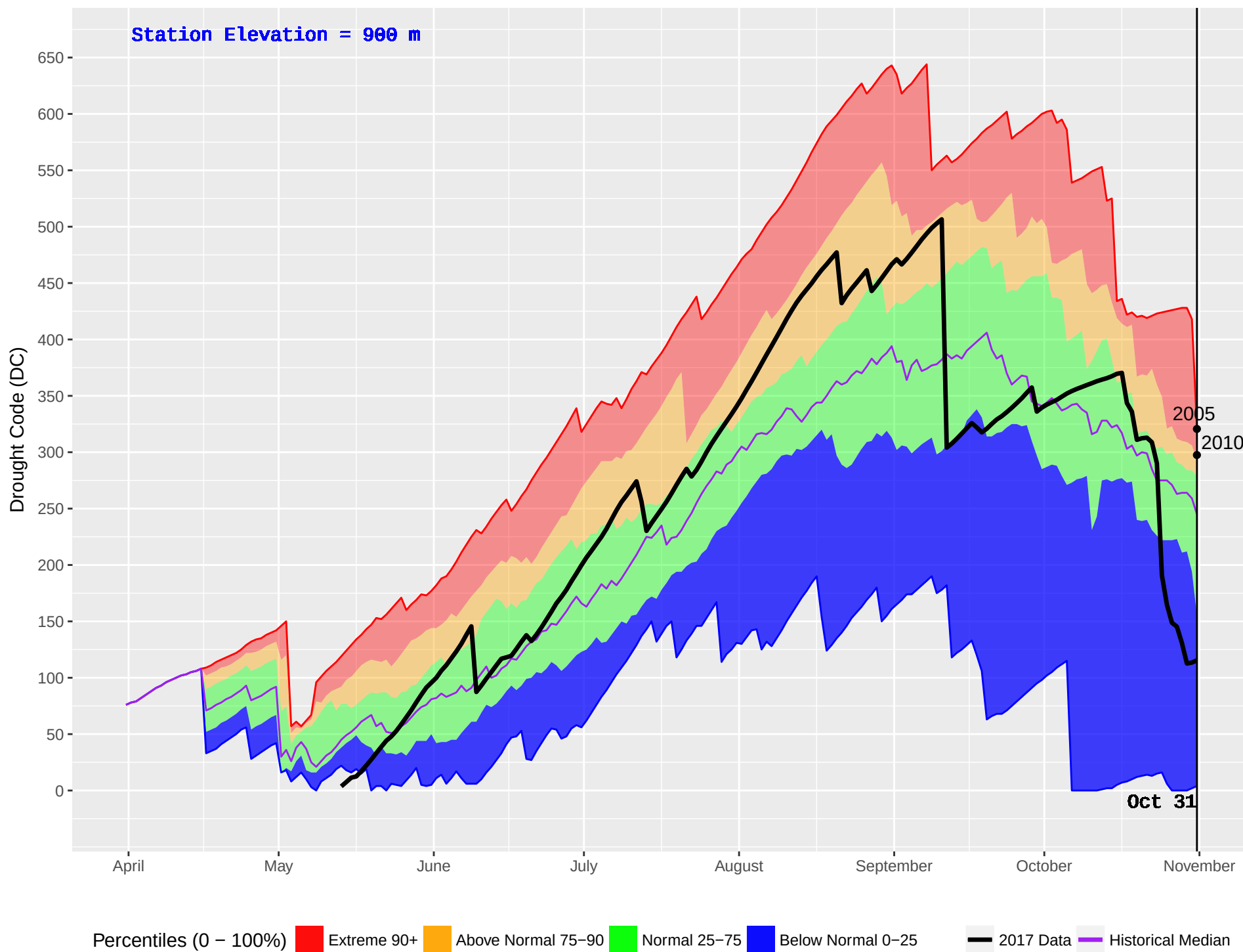
UPPER FULTON (169) : Historical (1986–2016) and Current (2017) Noon Drought Code (DC)
